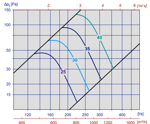
Diagram 26, UPK-R m / ATK-S 500x200 Ø315
