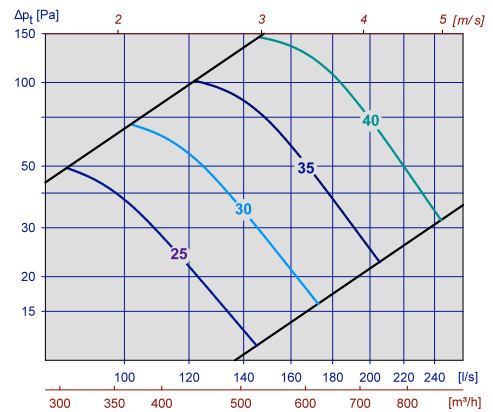
Diagram 24, UPK-R m / ATK-LS 400x200 Ø250
