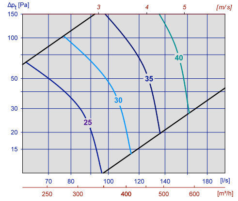
Diagram 10, UPK-R m / ATK-B 500x100 Ø160
