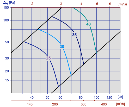
Diagram 6, UPK-R m / ATK-LS 300x100 Ø160
