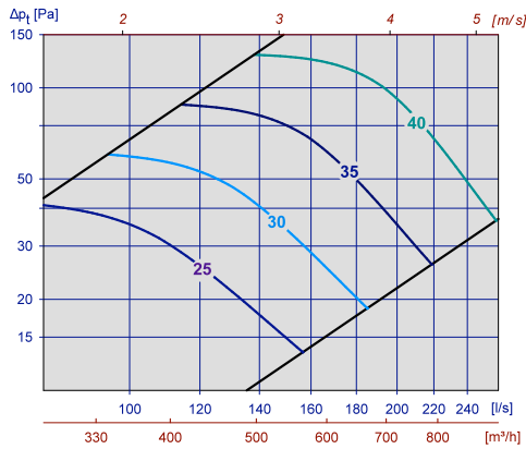
Diagram 23, UPK-R m / ATK-S 400x200 Ø250
