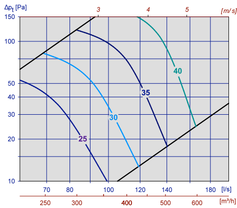
Diagram 13, UPK-R m / ATK-B 300x150 Ø200
