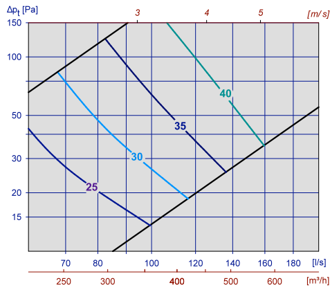
Diagram 11, UPK-R m / ATK-S 500x100 Ø200
