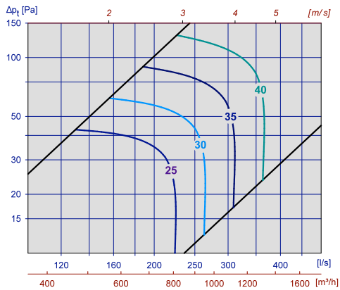
Diagram 25, UPK-R m / ATK-B 500x200 Ø315
