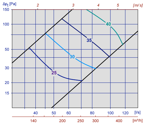
Diagram 9, UPK-R m / ATK-LS 400x100 Ø160
