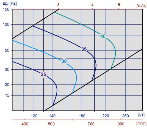
Diagram 21, UPK-R m / ATK-LS 500x150 Ø250
