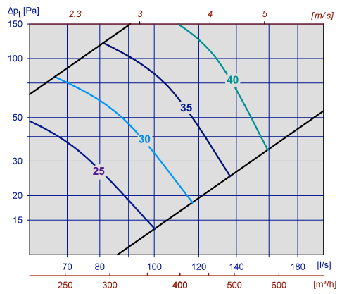
Diagram 14, UPK-R m / ATK-S 300x150 Ø200
