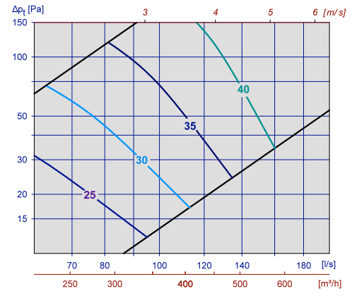
Diagram 12, UPK-R m / ATK-LS 500x100 Ø200
