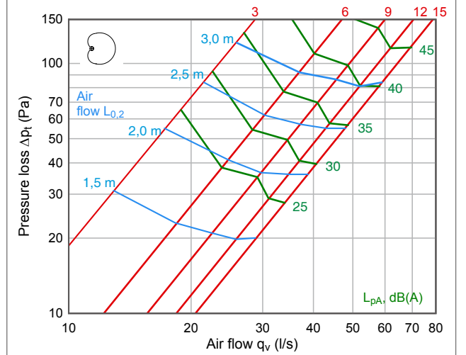
KSV 160 with sector plate
