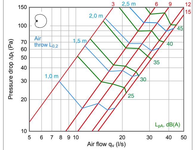
KSV 125 with sector plate
